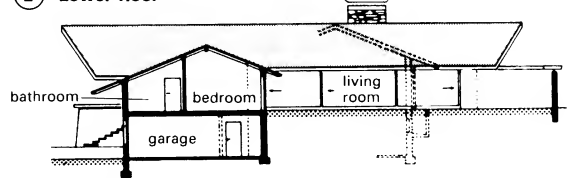
5 Section
